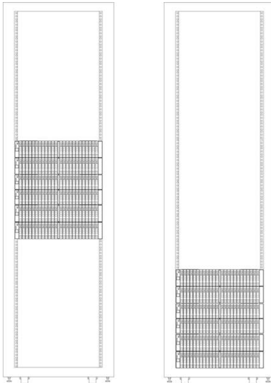
StoreServ 8000 4-node Storage system in a storage centric configuration in a HPE Intelligent Series Rack
