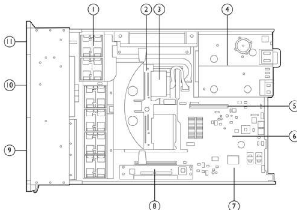
HPE Integrity rx2800 i4 Server: Inside View
