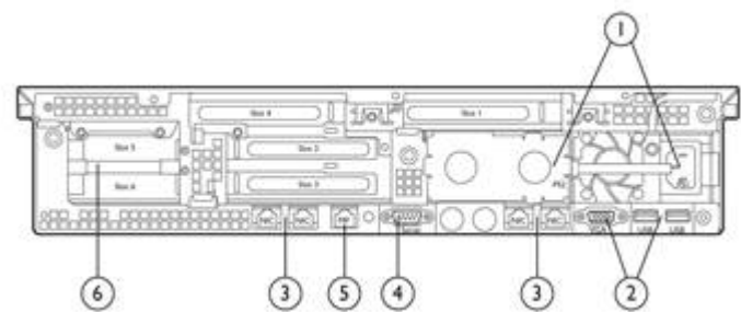
HPE Integrity rx2800 i4 Server: Rear View
